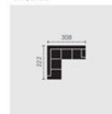
C439759 OTM/ST-2.5
